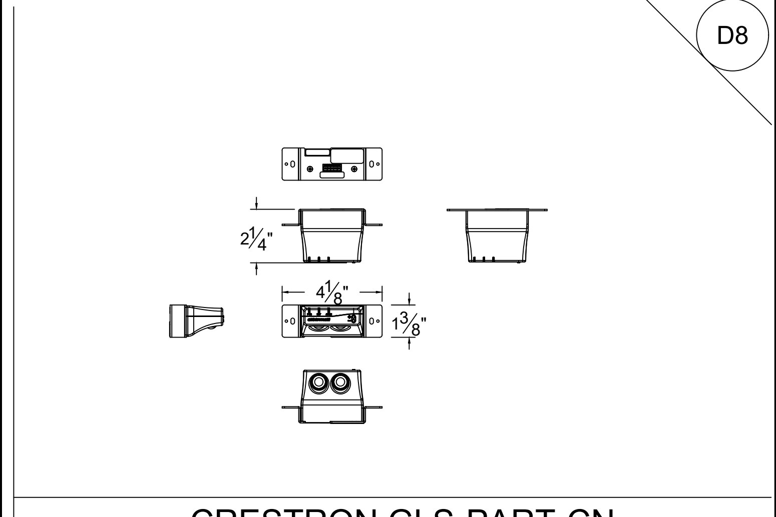
CRESTRON GLS-PART-CN
