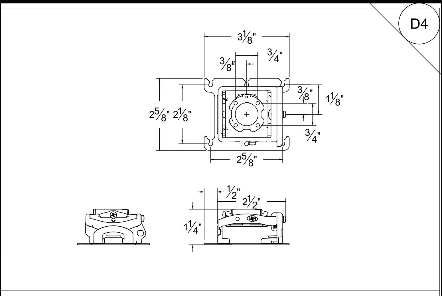
CHIEF RPMAUW
