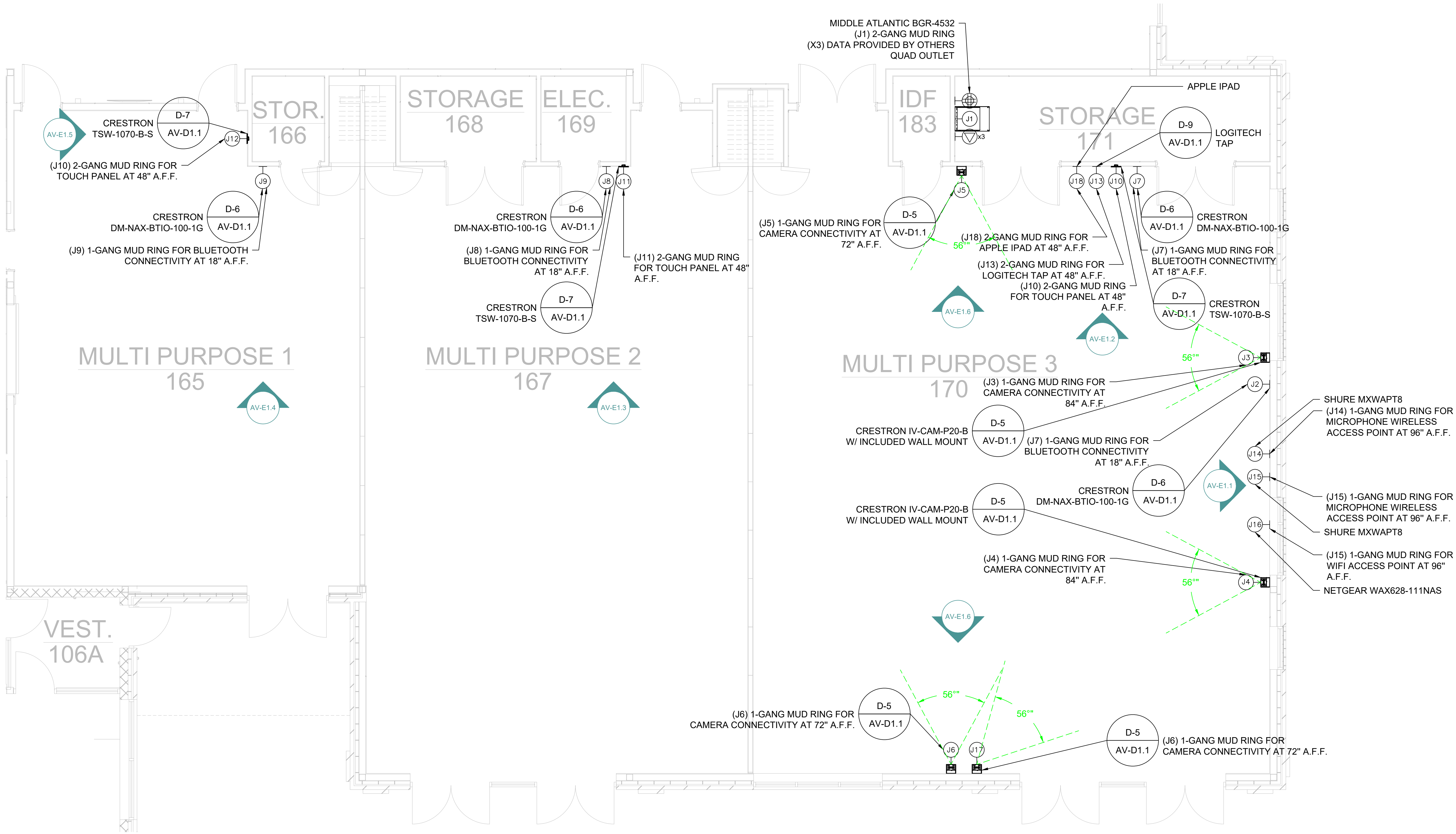
1 MULTIPURPOSE 1 ROOM 165, MULTIPURPOSE 2 ROOM 167 & MULTIPURPOSE 3 ROOM 170 - FLOOR PLAN SCALE: 1/4"=1'-0" ARCH D
