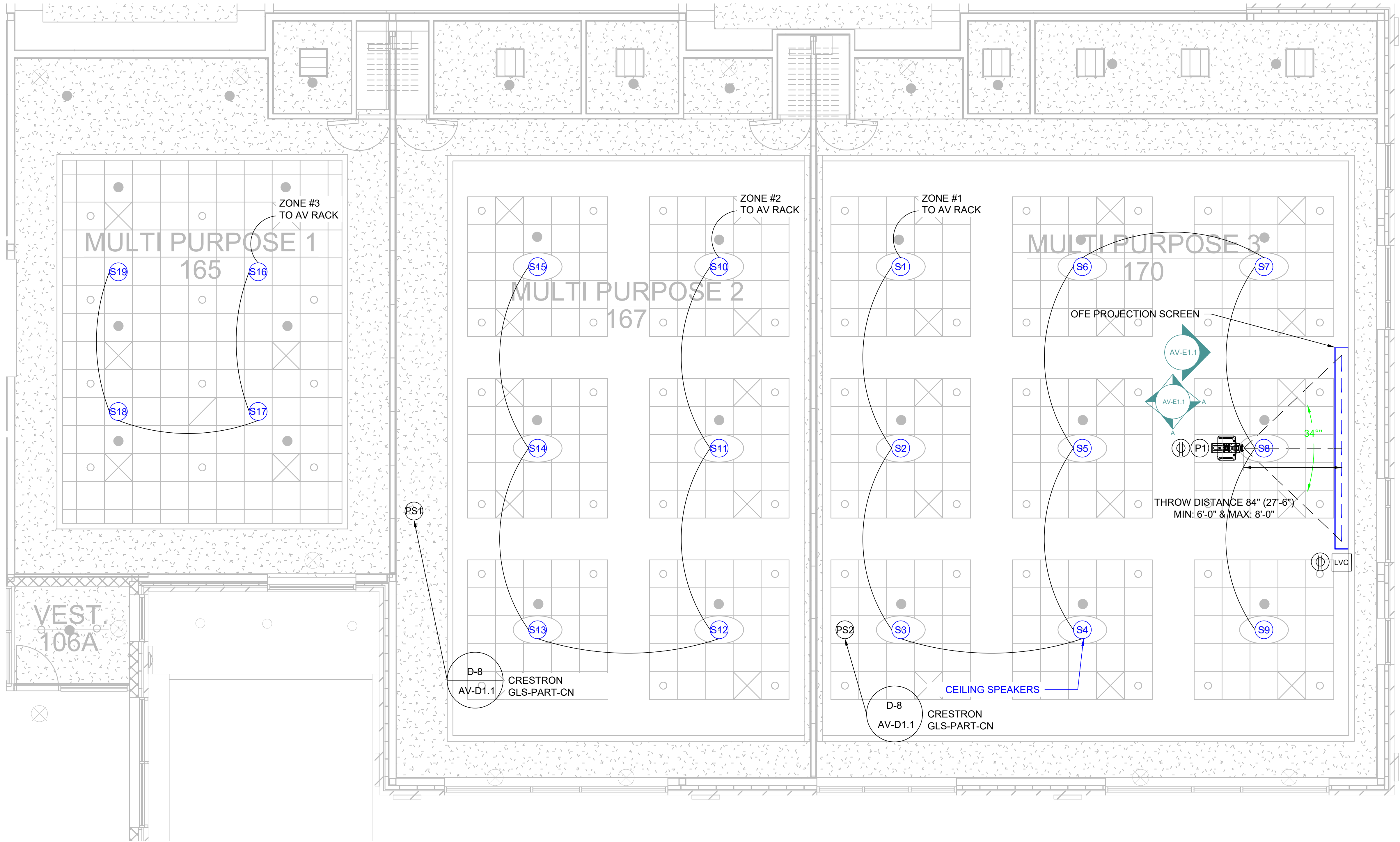
1 MULTIPURPOSE 1 ROOM 165, MULTIPURPOSE 2 ROOM 167 & MULTIPURPOSE 3 ROOM 170 - CEILING PLAN SCALE: 1/4"=1'-0" ARCH D
