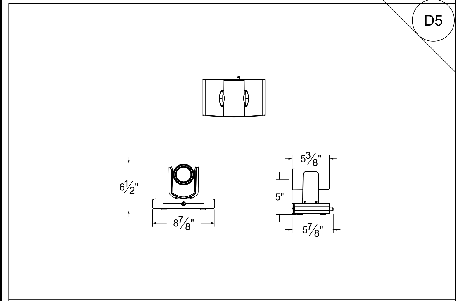
CRESTRON IV-CAM-P20
