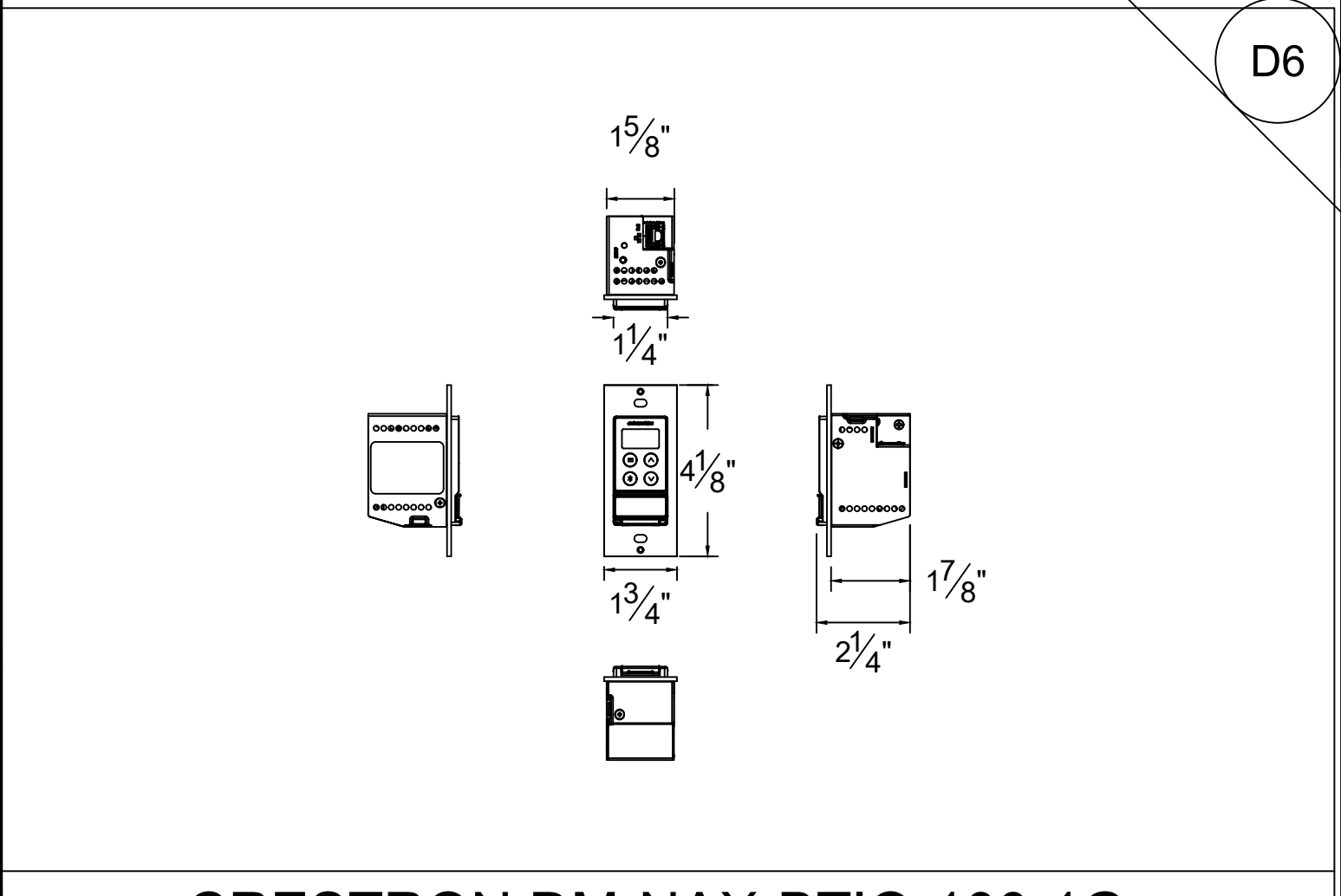
CRESTRON DM-NAX-BTIO-100-1G
