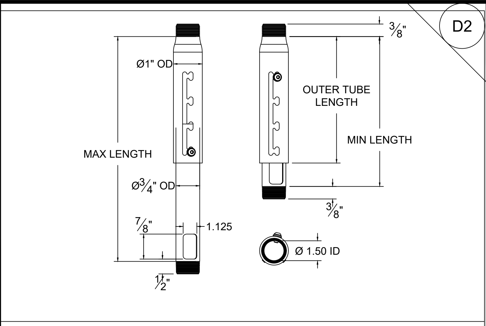
CHIEF CMS0305W
